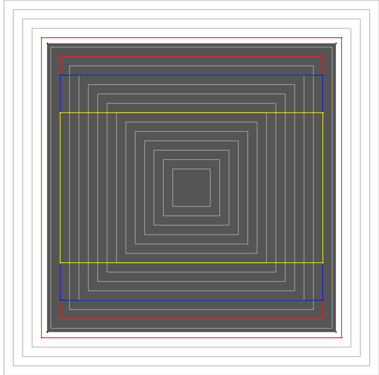
Figure 13.8 fullsquare
