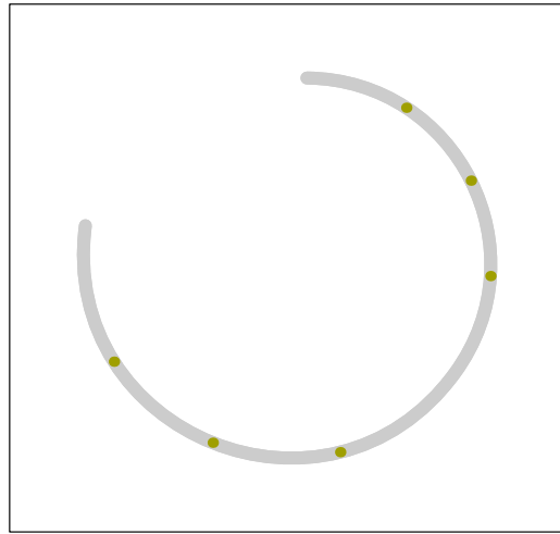
second iteration
