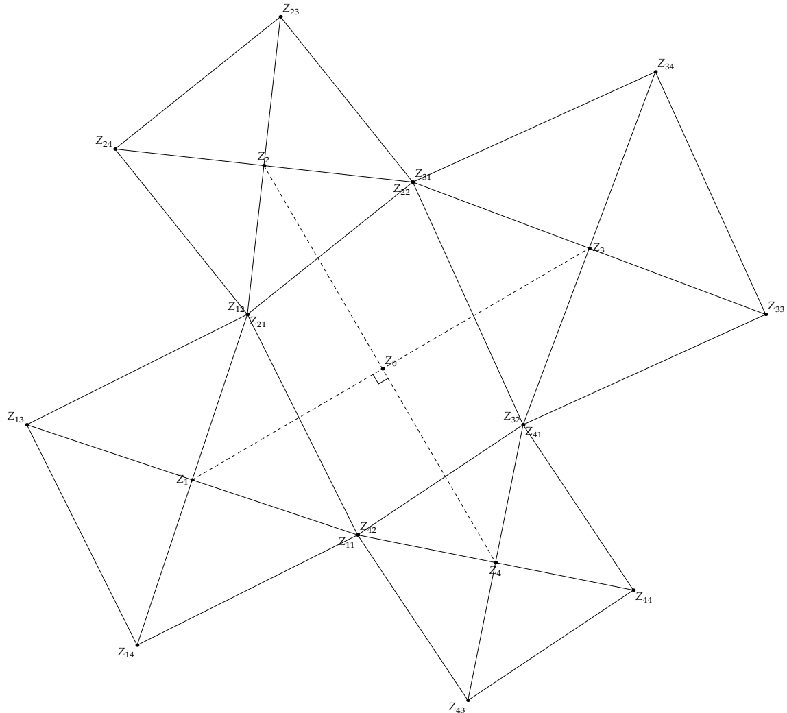
Figure 1.4 The problem.
