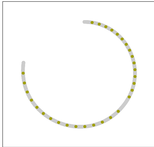
fourth iteration
