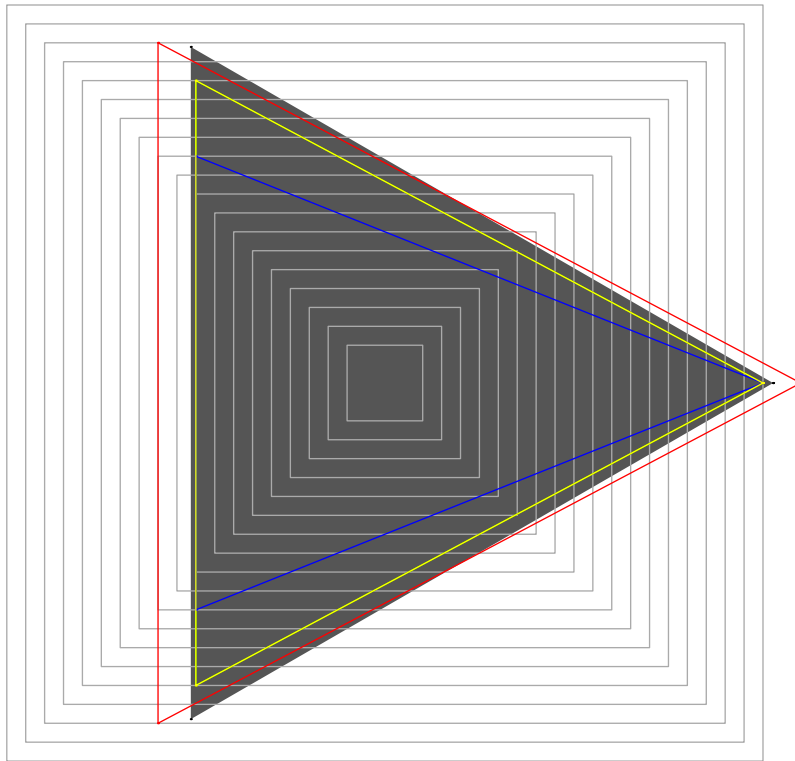
Figure 13.9 fulltriangle
