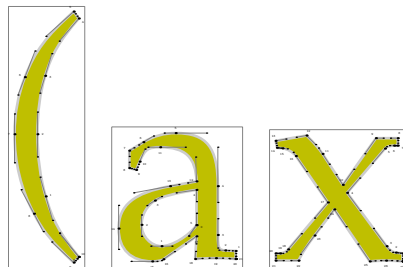
Figure 8.15 Showing shapes.
