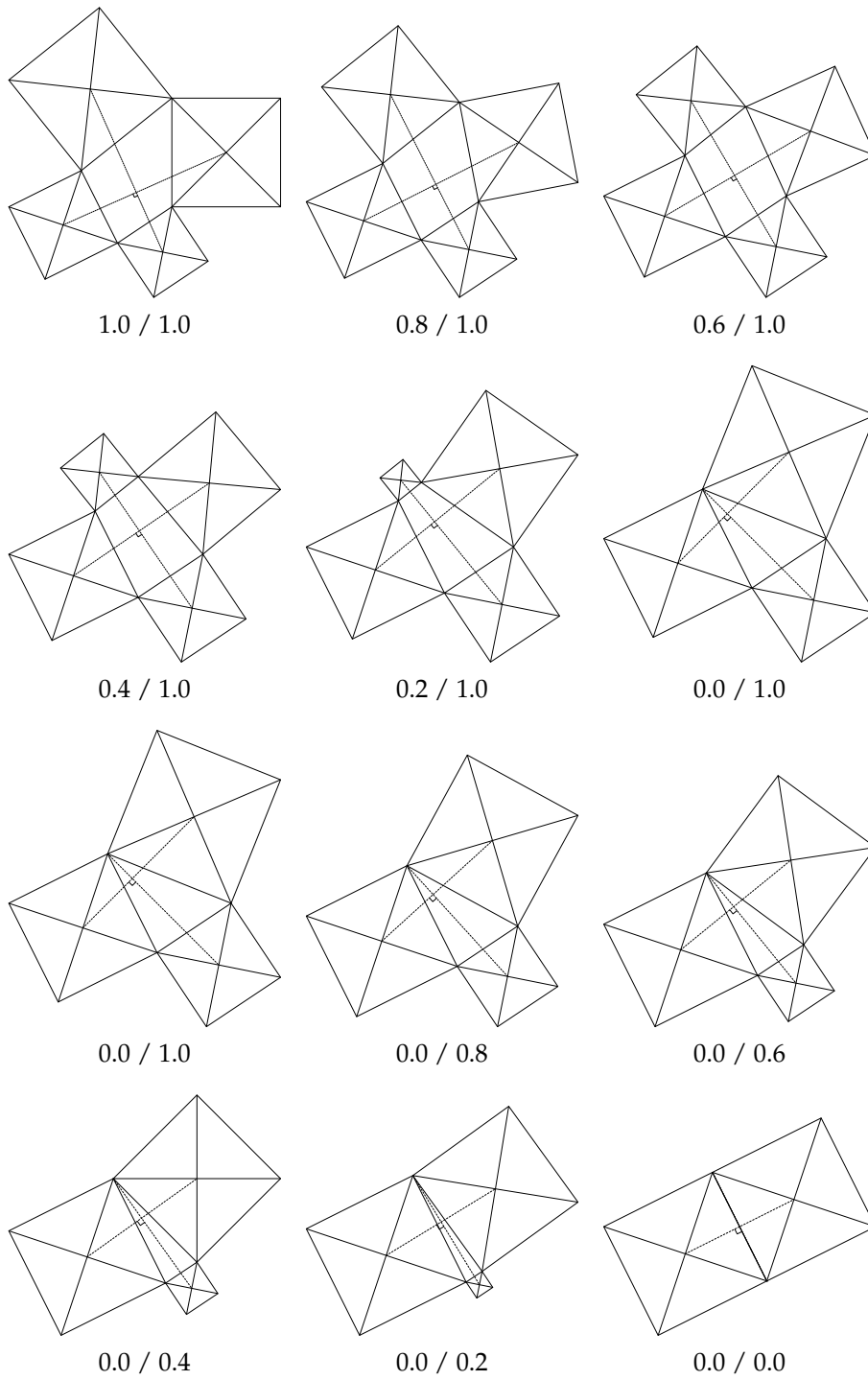
Figure 1.5 The solution.
