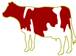
Figure 8.5 A cow.
